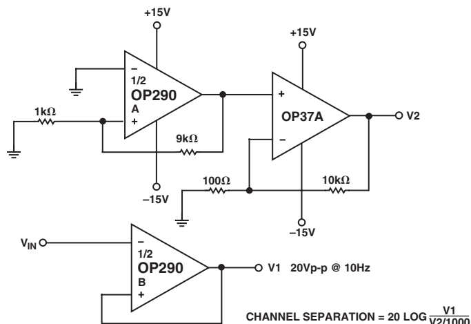
Figure 3. Channel Separation Test Circuit
